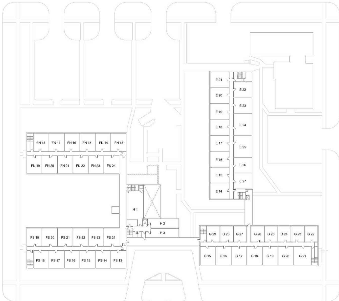
Port Huron Housing Commission Desmond Village - Senior Housing 2nd Floor Plan
